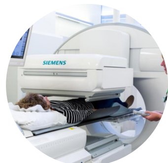
SPECT Scan
